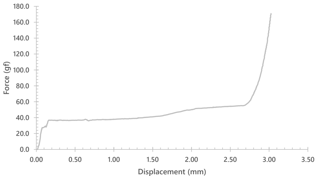
Gateron KS-33 Low Profile Silent Red (Upstroke)
